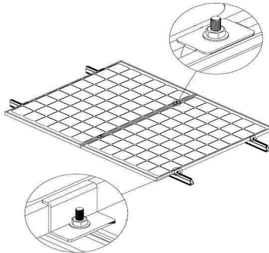
Picture 2.11: Solar panels installed with appropriate equipment
