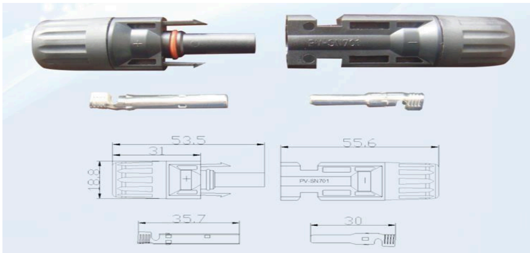
Picture 3.4: Male and female solar cable connector
