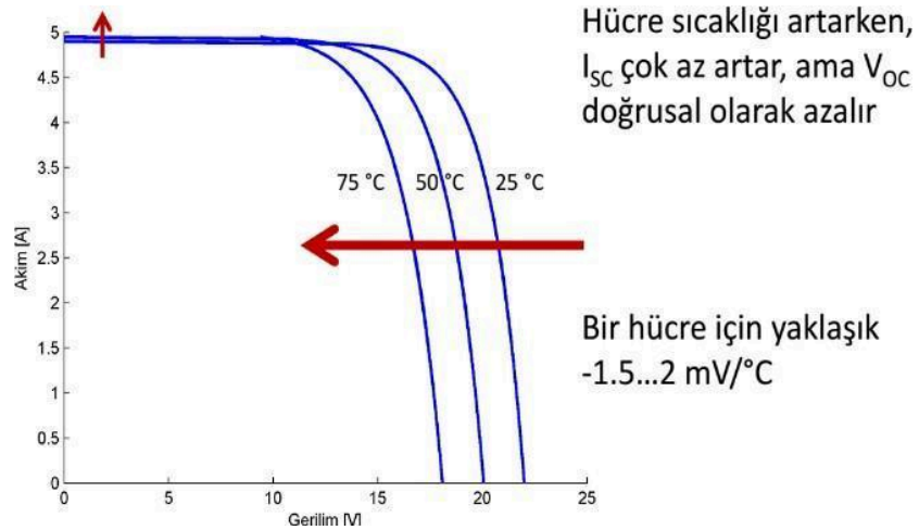
Figure 2.3: Change of current and voltage depending on temperature
